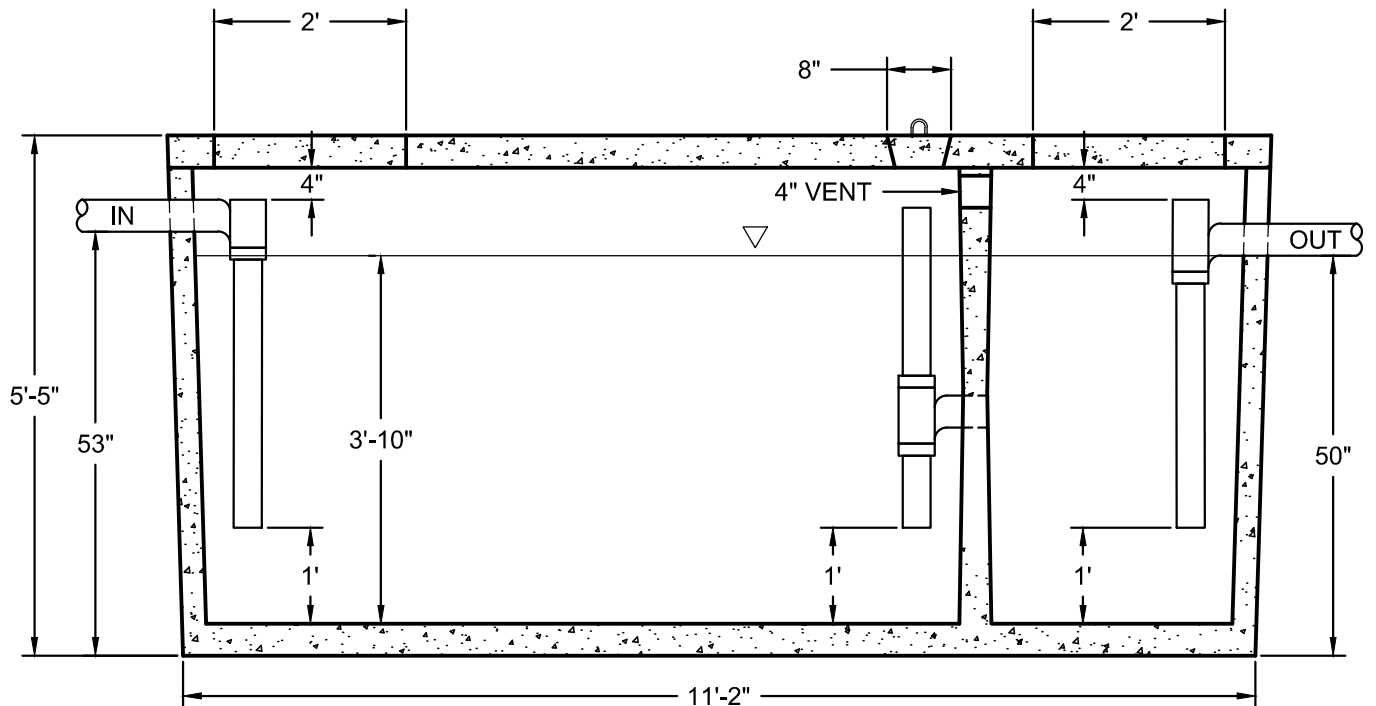
SECTION VIEW
