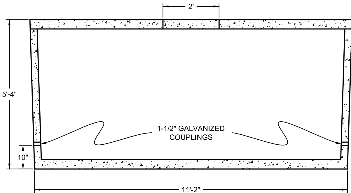
SECTION VIEW
