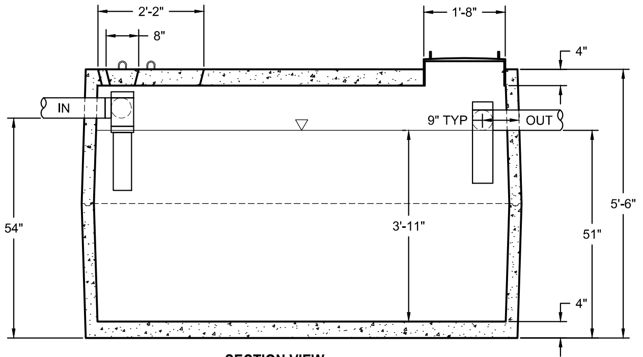
SECTION VIEW
