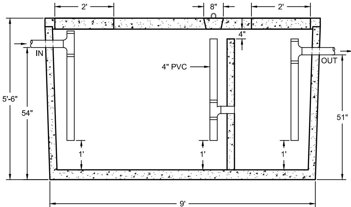
SECTION VIEW
