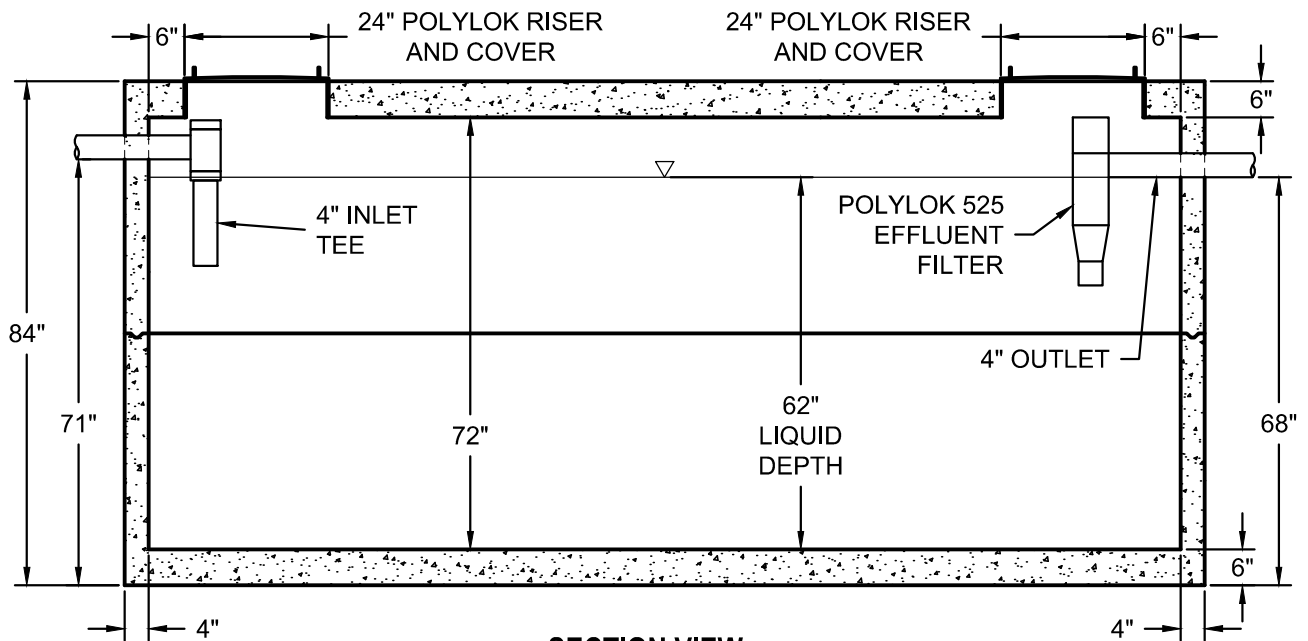
SECTION VIEW
