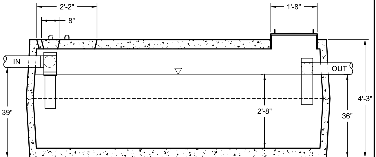
SECTION VIEW
