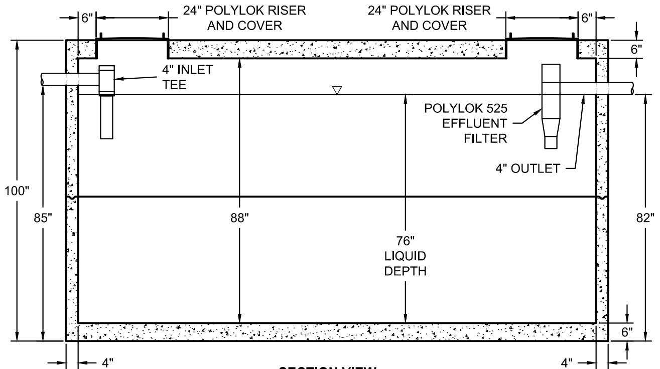
SECTION VIEW
