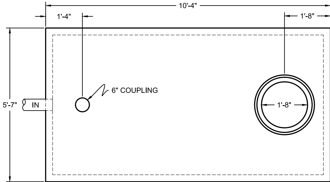
PLAN VIEW
