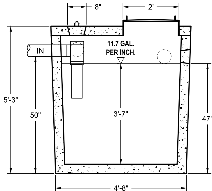
SECTION VIEW
